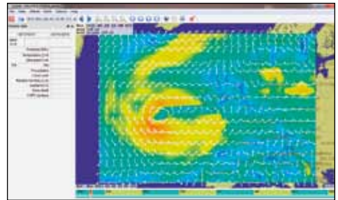
zyGrib-Software
